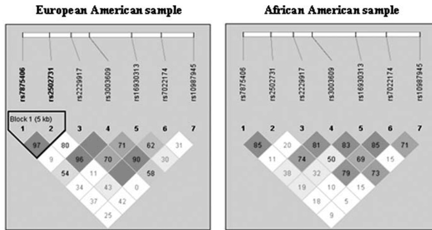
Figure 1 Haploview-generated linkage disequilibrium (LD) maps of the seven single-nucleotide polymorphisms (SNPs) within dynamin I gene ( DNM1 ) in the European-American (EA) and African-American (AA) samples. Regions of high LD ( D = 1 and LD > 2 ) are shown in dark gray. Markers with LD ( 0.21 < D < 1 and LOD > 2 ) are shown in dark through light gray, with the color intensity decreasing with decreasing D values. Regions of low LD and low LOD scores ( LOD < 2 ) are shown in white. The number within each box indicates the D statistic between the two SNPs. Haplotype blocks in the two samples were produced by the HaploView program using the block definitions proposed by Grabiell et al.
