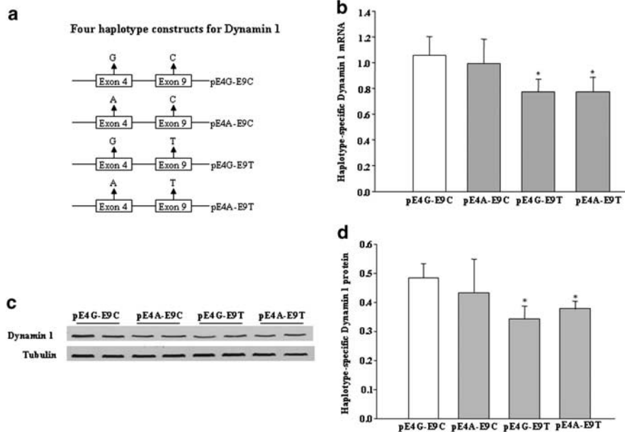
Figure 2 Expression analyses of allele combinations of single-nucleotide polymorphisms (SNPs) rs2229917 at exon 4 and rs3003609 at exon 9. (a) Illustration of four plasmids constructed for dynamin 1 expression analysis. (b) Statistical analysis of real-time RT-PCR data for the four plasmids. 18S RNA was used to normalize expression of each dynamin 1 gene ( DNM1 ) construct. Compared with pE4G-E9C, pE4G-E9T and pE4A-E9T showed lower expression of dynamin 1, by 27.1 and 26.8%, respectively. No significant difference was detected between constructs pE4G-E9C and pE4A-E9C. (c) Representative western blotting images for dynamin 1 and tubulin. Tubulin was used to normalize expression of each DNM1 construct. (d) Statistical analysis of the protein expression levels of four DNM1 constructs. Similar to the mRNA expression data in (c), pE4G-E9T and pE4A-E9T showed decreased dynamin 1 protein expression, by 29.2 and 22.2%, respectively, compared with pE4G-E9C. Data in b and d are given as means \pm SEM (* P < 0.05 ; n = 3 per group).
