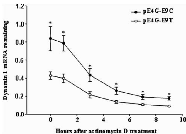
Figure 3 Comparison of mRNA stability of dynamin 1 gene ( DNM1 ) from pE4G-E9C and pE4G-E9T constructs. Measured half-life of mRNA was about 3.2 h for the former and 3.6 h for the latter. No significant difference in the half-life of DNM1 mRNA was found in the two constructs. Data are given as means \pm SEM (* P < 0.05 ; n = 3 per group).
